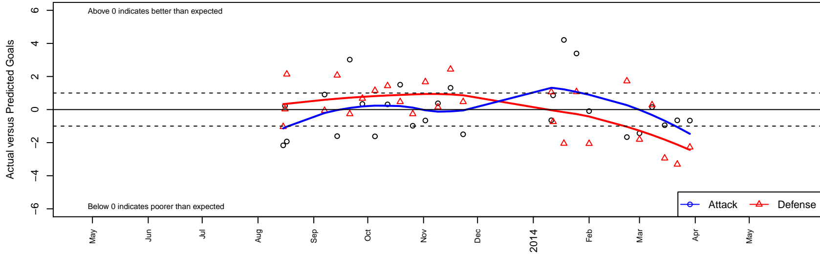
Newport FC Tango G02 Dots are actual minus expected GF (blue circles) and GA (red triangles). Blue line is smoothed change in attack strength. Red is smoothed change in defense strength.
